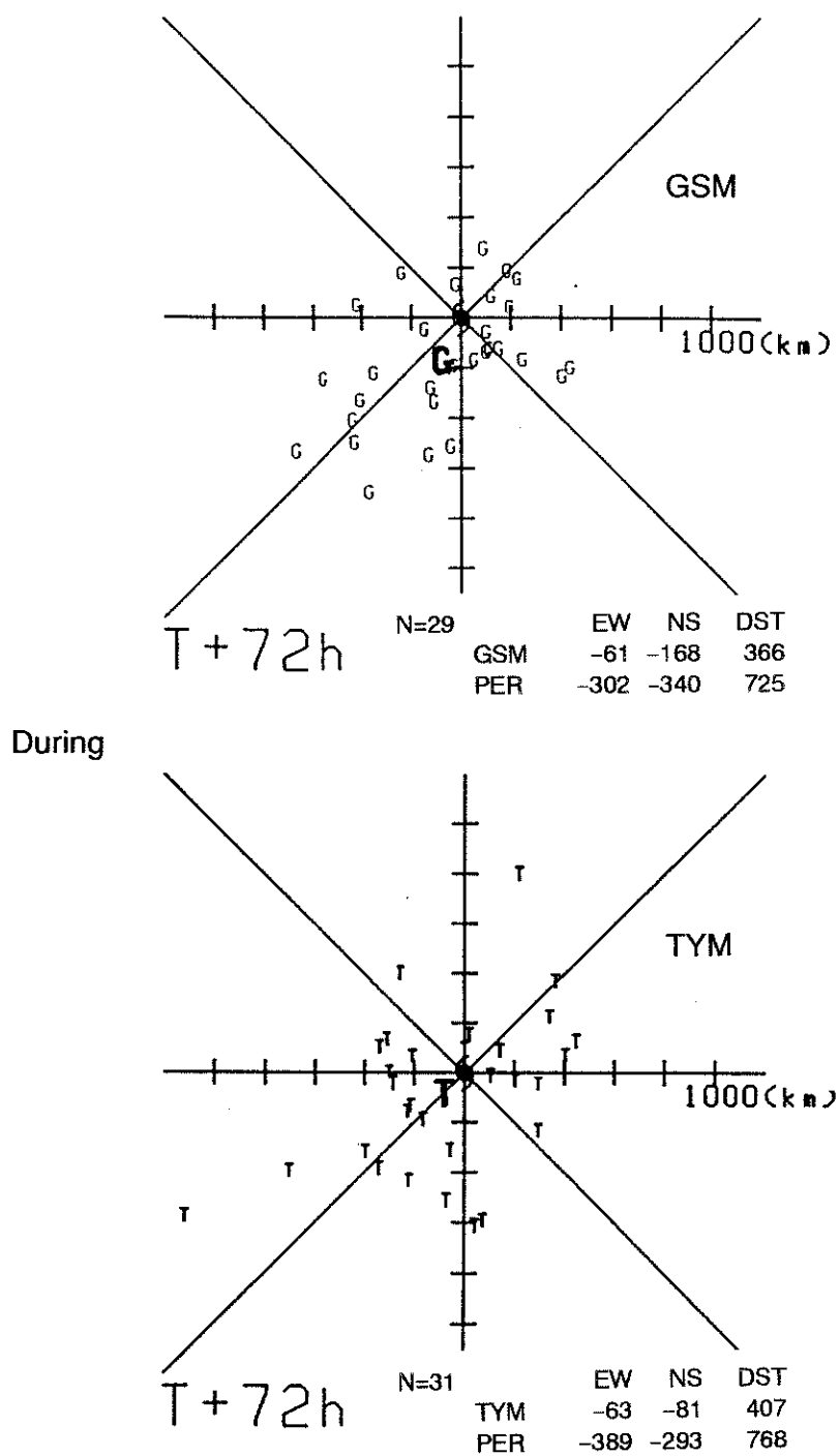
Figure 2(b) Same as in Figure 2(a) except for the stage "During recurvature".
