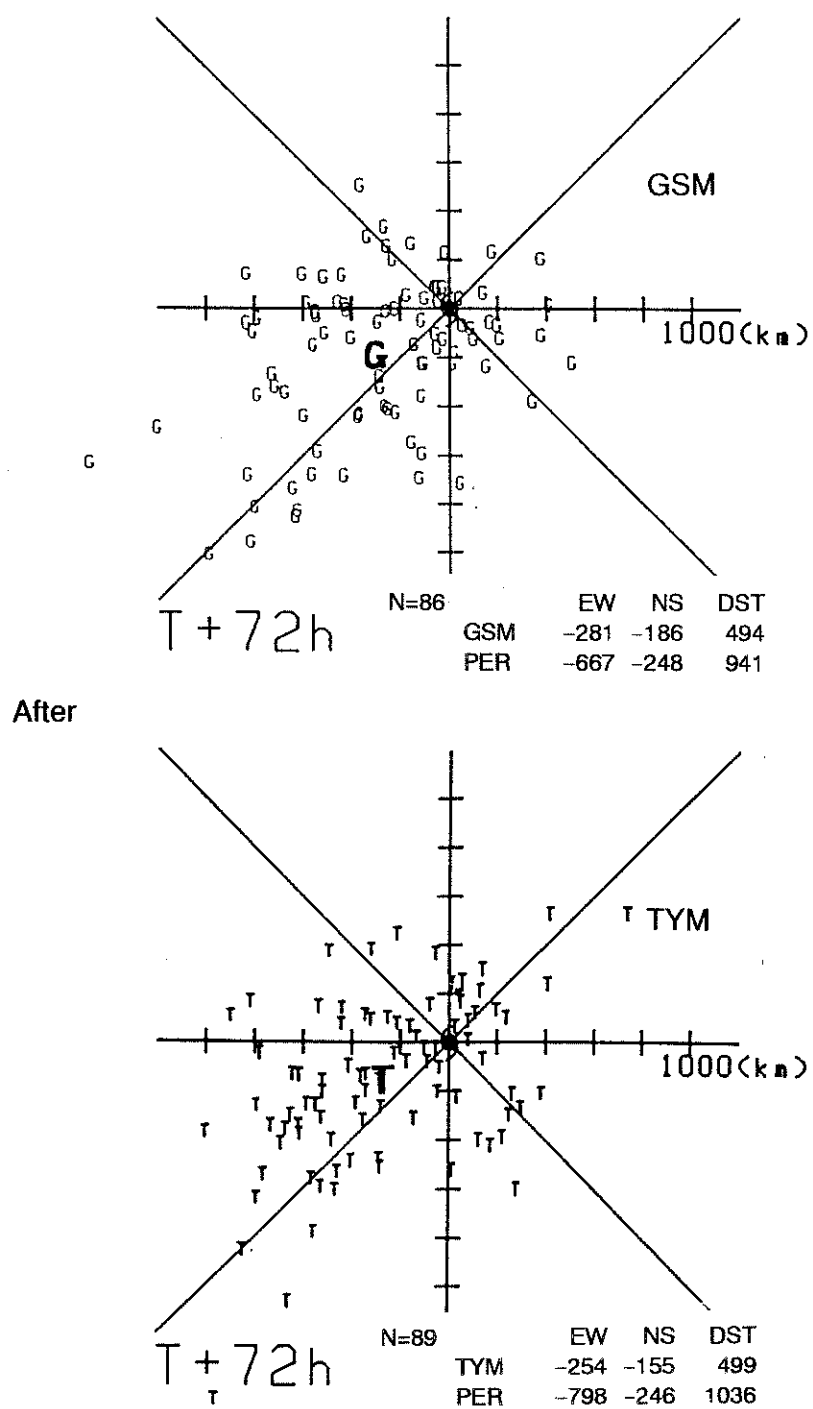
Figure 2(c) Same as in Figure 2(a) except for the stage "After recurvature".
