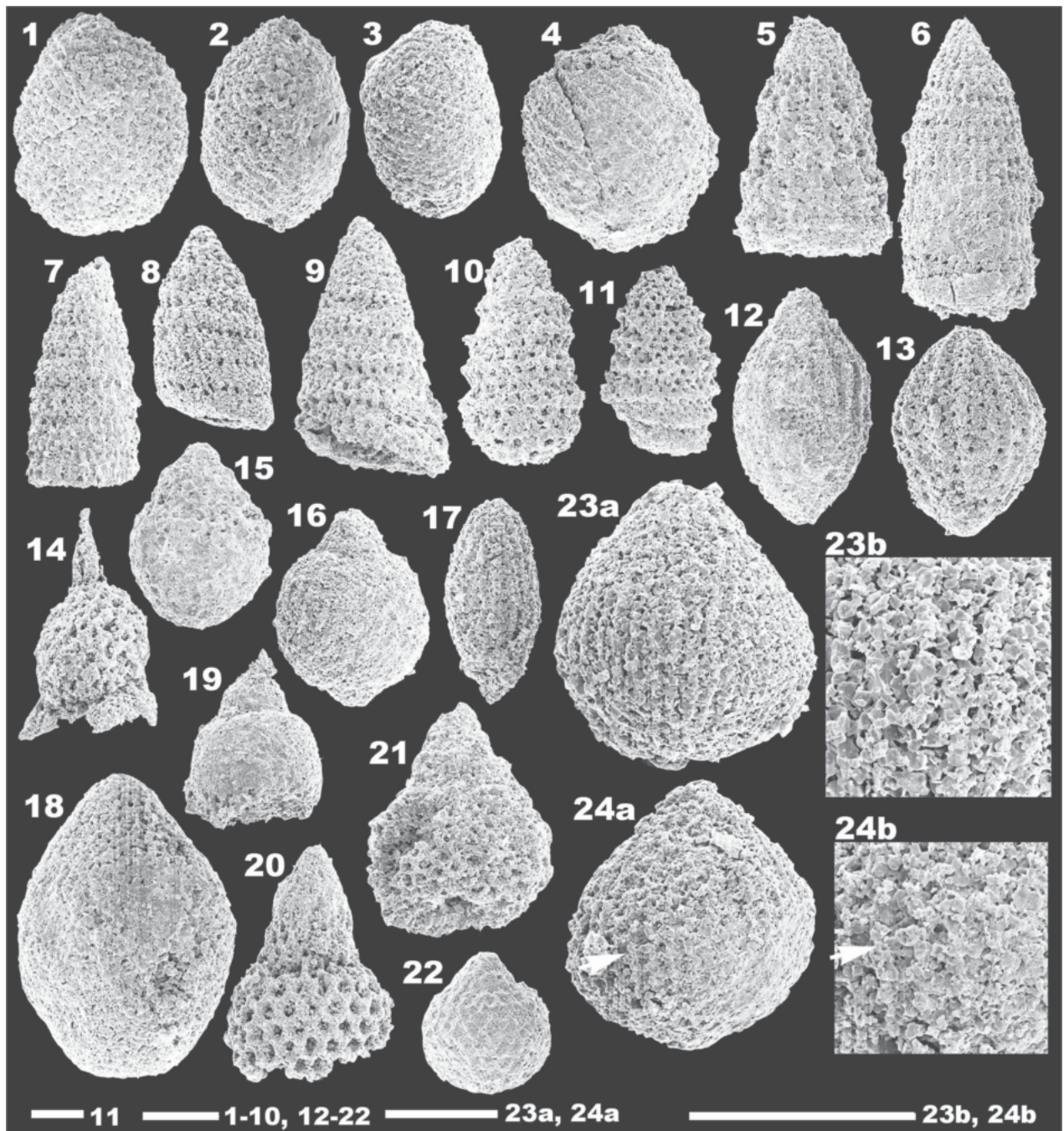
FIGURE 4. SEM photographs of the latest Middle to early Late Jurassic radiolarians obtained from the bore-hole core sample. All scale bars indicate 50µm. 1–4, Stylocapsa (?) spiralis ; 5, Hsuum sp.; 6, Archaeodictyomitra sp.; 7, Loopus (?) sp.; 8, Loopus sp.; 9, Dictyomitrella (?) kamoensis ; 10, Amphipyndax durisaepum ; 11, Parvicingula sp.; 12, Protunuma japonicus ; 13, Protunuma (?) ochiensis ; 14, Triactoma sp.; 15, Zhamoidellum ovum ; 16, Tricolocapsa sp.; 17, Stylocapsa sp. cf. S. catenarum ; 18, Stichocapsa robusta ; 19, Eucyrtidiellum sp.; 20–21, Sethocapsa spp.; 22, Tricolocapsa sp.; 23a–b, Tricolocapsa plicarum s.l.; 24a–b, Tricolocapsa conexa . Arrows indicate transverse ridge.
