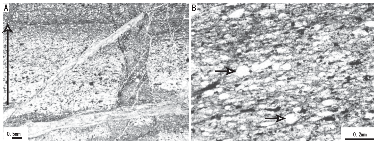
FIGURE 3. Photomicrographs of alternating thin beds of sandstone and siltstone. The photographs were taken under plane-polarized light. A, Arrow indicates grading from fine-grained sandstone to siltstone; B, Many radiolarian fossils are scattered within the siltstone. Arrows indicate radiolarians.
