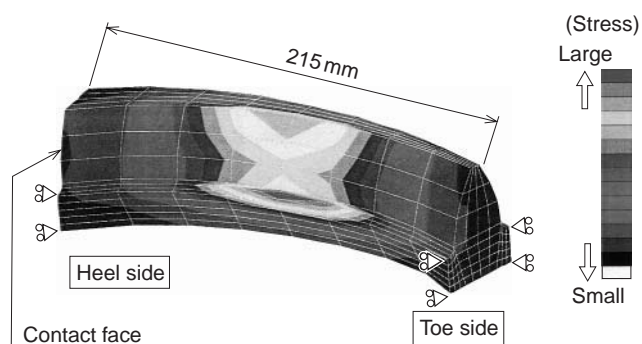
Fig. 11 Bending stress analysis on a spiral bevel gear
