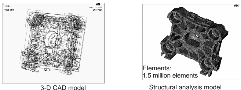
Fig. 6 Die head of injection molding machine
