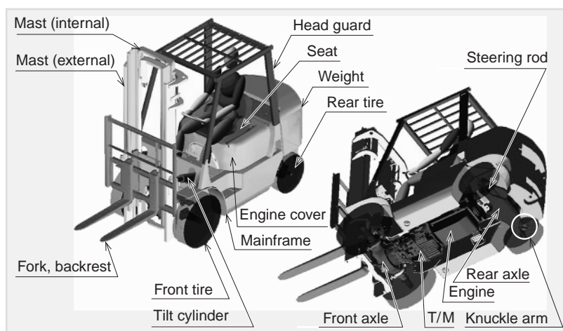
Fig. 7 Multibody dynamics model of forklift truck
