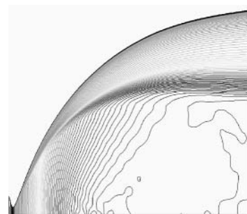
Fig. 14 Mach-number contour in a supersonic wind tunnel (the scale in the radial direction is magnified by a factor of ten) MHI has developed a nozzle that generates decreased fluctuations by grasping the weak compression waves inside a nozzle using an advanced precision numerical method, and utilizing CFD.
