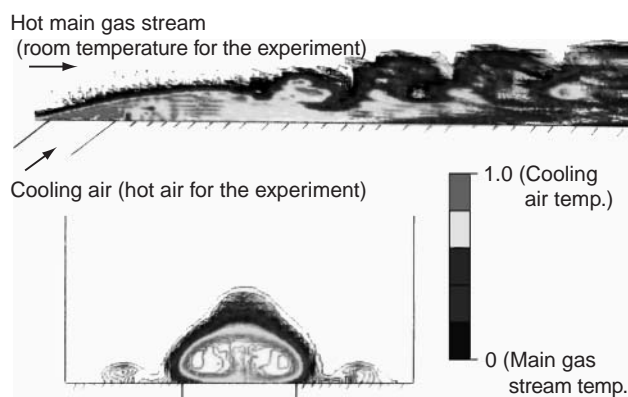
Fig. 18 LES analysis of film cooling: mixing of air-film with main gas stream
