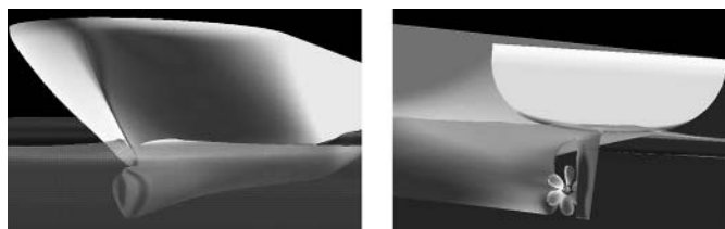
Fig. 13 Integrated fluid analysis of hull and propeller
