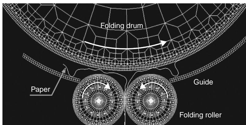
Fig. 8 Analysis of mechanism to prevent edge folding in paper folding machine
