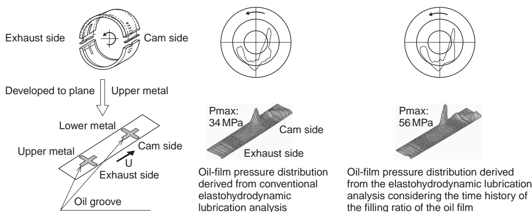
Fig. 9 Computation of oil-film pressure distribution in an engine bearing
