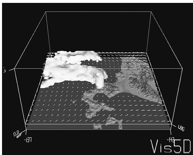
Fig. 12 Prediction of smoke diffusion from Mt. Usu.
