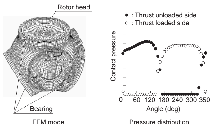
Fig. 10 Structure of windmill bearing and rotor head; pressure distribution derived from the combined analysis of FEM of the structure with the numerical model of the bearing
