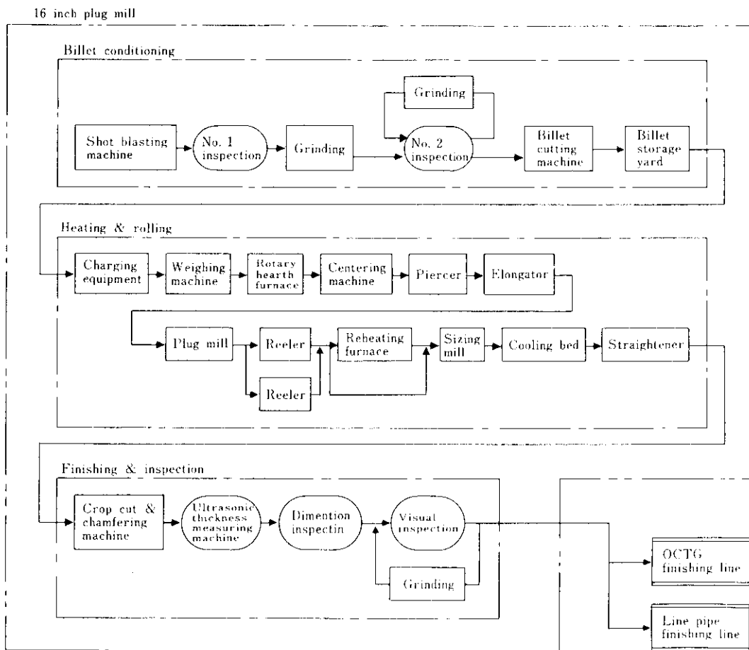
Fig.1 Manufacturing process of 16-inch plug mill
