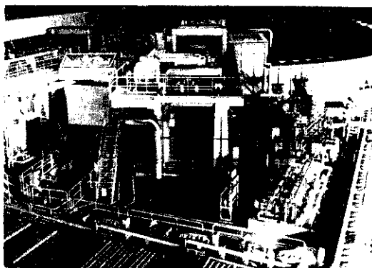
Photo.1 Rotary hearth furnace
