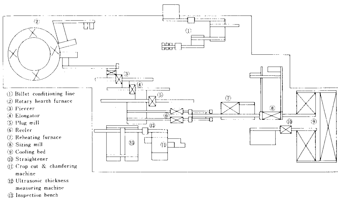
Fig.2 Layout of 16-inch plug mill
