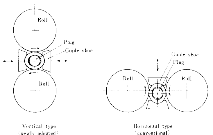
Fig.5 Arrangement of piercer rolls
