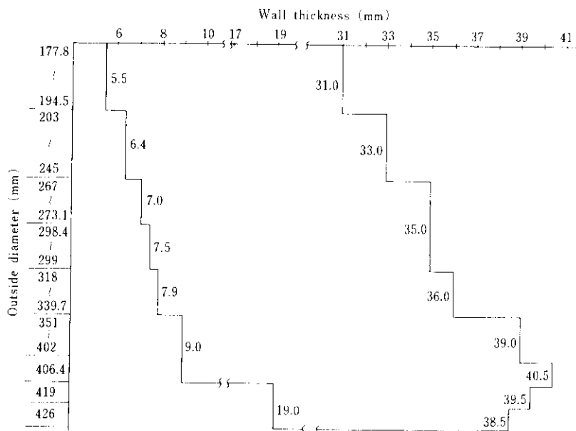
Fig.4 Size available at 16-inch plug mill
