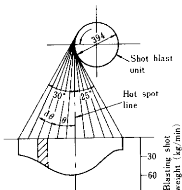
Fig. 2 Blasting shot distribution of one shot blast unit
