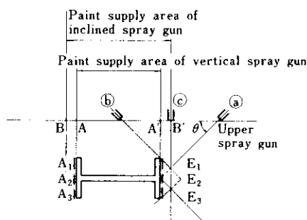
Fig. 12 Painting range of spray guns
