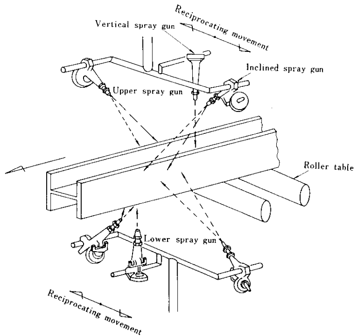
Fig. 9 Tripple gun system
