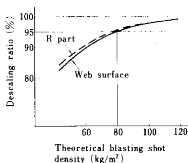
Fig. 5 Relation between descaling ratio and blasting shot density
