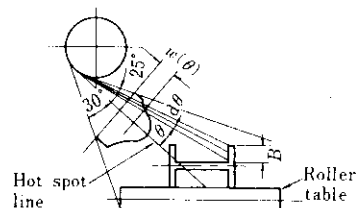
Fig. 3 An example of blasting pattern on H-shapes
