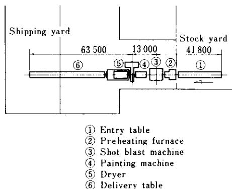
Fig. 1 Layout of the automatic shot blast and spray painting line
