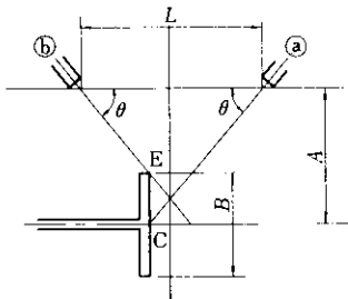
Fig. 14 Inclined guns position adjusting method
