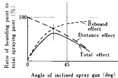
Fig. 10 Relation between ratio of bounding paint to total spraying paint and inclined angle
