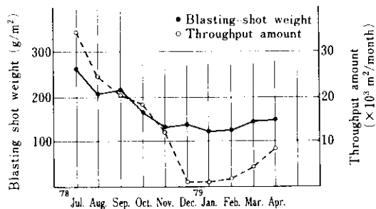
Fig. 8 Throughput amount and blasting shot weight
