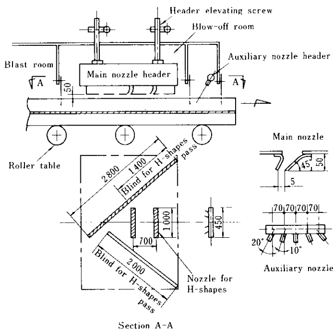
Fig. 7 Shot blow-off mechanism
