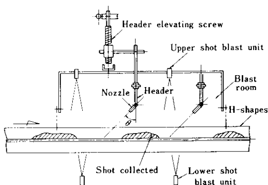
Fig. 6 Air blowing header in blast room
