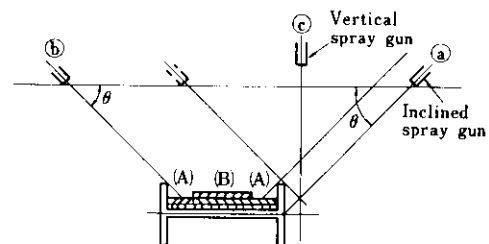
Fig. 11 Schema of paint film thickness on web surface by tripple spray gun system
