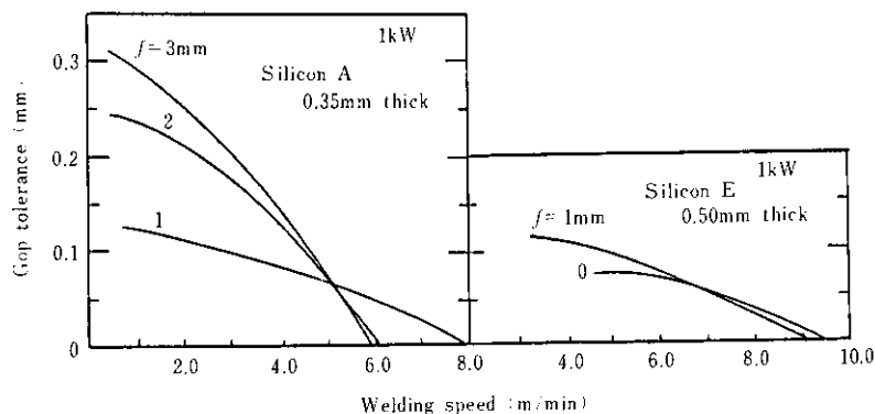
Fig. 7 Variation of gap tolerance with focus deviation and welding speed
