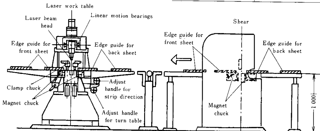
Fig. 13 Laser welding machine
