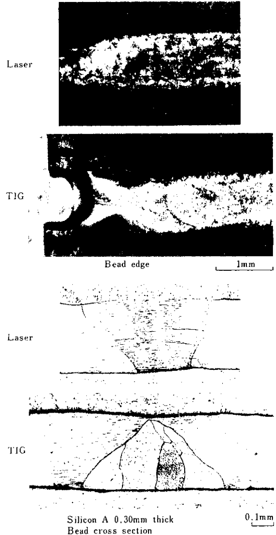
Photo. 1 Appearance of Laser and TIG welded joints
