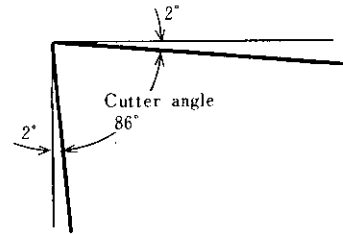
Fig. 11 Cutter angle
