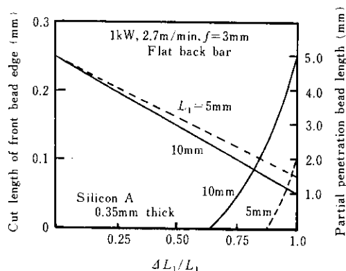
Fig. 9 Relation between bead shapes and power control parameter( \Delta L_1/L_1 )
