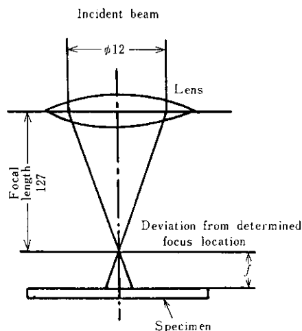
Fig. 2 Dimensions of focusing system
