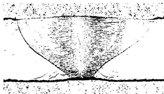
Bead cross section
