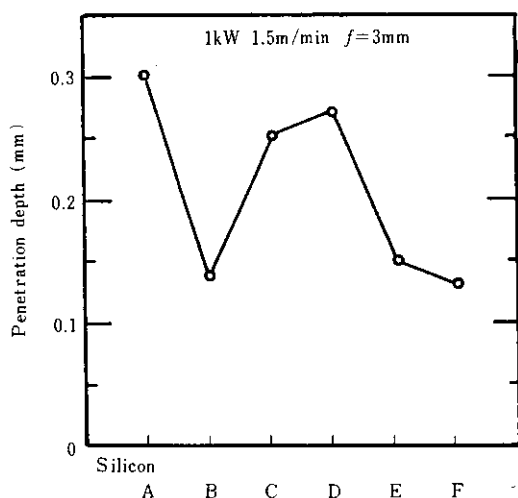
Fig. 3 Variation of penetration depth with materials and thickness of coatings
