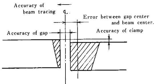
Fig. 10 Factors of fit-up and alignment accuracies
