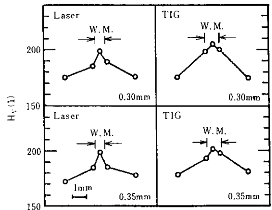
Fig. 1 Hardness distribution in welded joint
