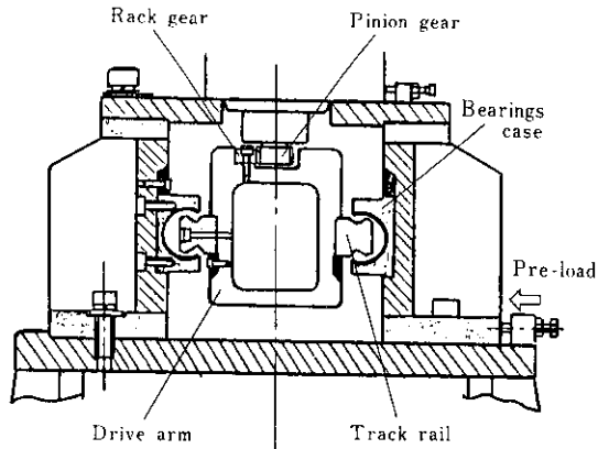
Fig. 12 Laser beam head traversing mechanism
