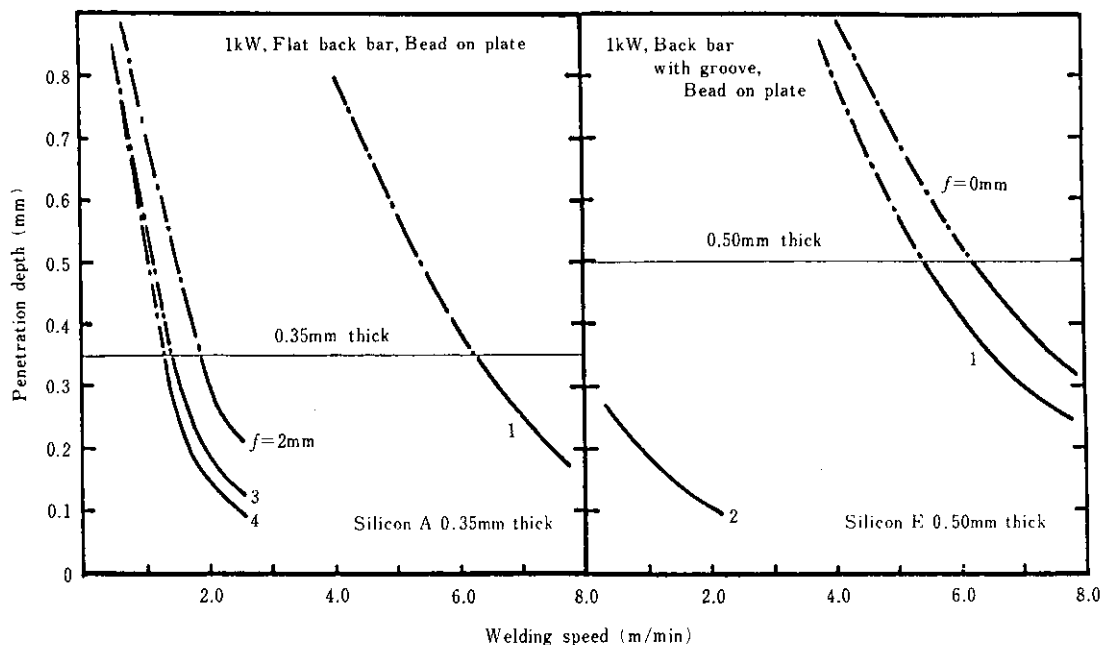
Fig. 4 Variation of penetration depth with focus deviation and welding speed
