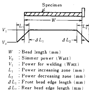
Fig. 8 Schematic diagram of power controll for edge shaping
