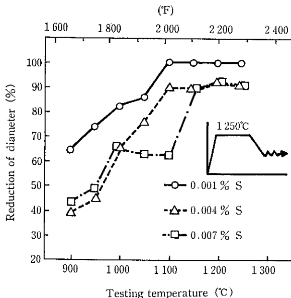
Fig. 2 Effect of S-content on hot workability of 13% Cr stainless steel
