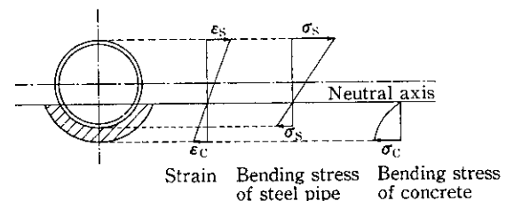
Fig. 9 Model of composite pipe
