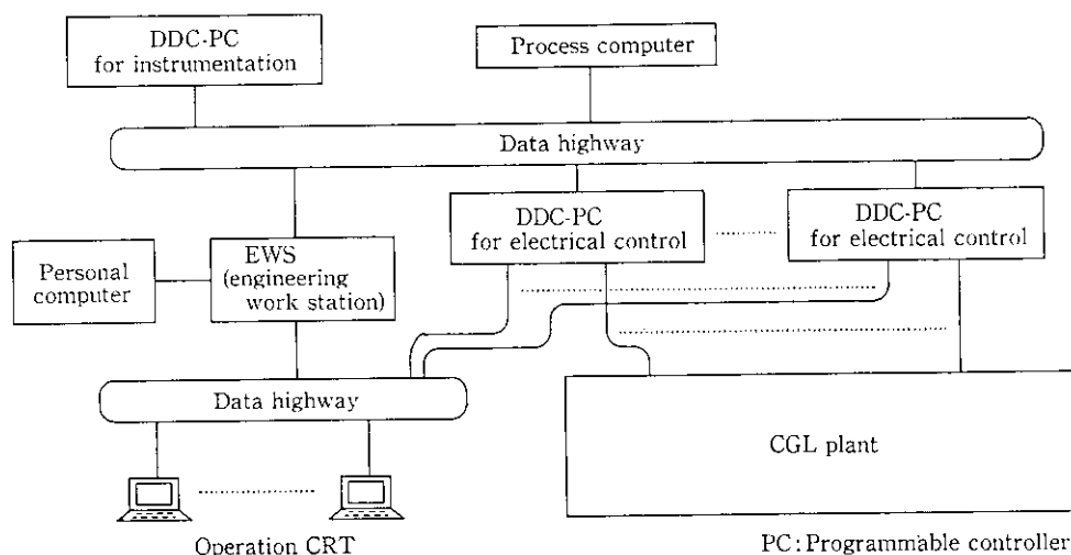
Fig. 2 Control system of the CGL plant at Mizushima Works
