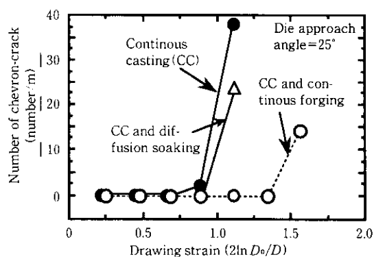
Fig. 8 Relationship between drawing strain and number of chevron-crack of SWRH82A
