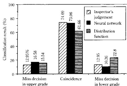
Fig. 6 Experimental results of the glossiness evaluation
