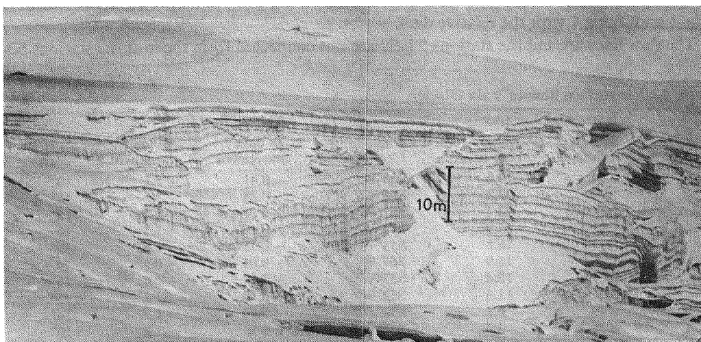
Fig. 4. Ice cliffs (G) below the boring site (BS: altitude 5405 m, upper-left in the picture).
