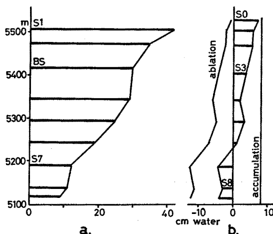
Fig. 3. Profiles of mass balance against altitude.
