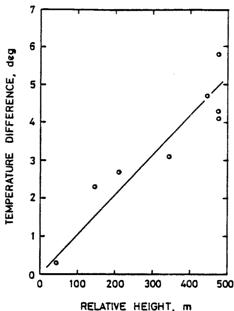
Fig. 2. Temperatures at different elevations. The linear least square fit gave the lapse rate 1.05^{\circ}\text{C}/100\text{ m} .
