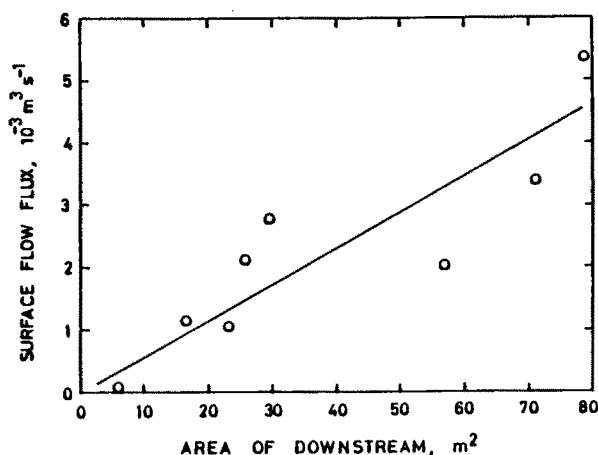
Fig. 5. Surface flow flux versus the area of the stream between the observation site and the stream terminus. The linear least square fit to the data gave a vertical water flow flux of 58 \times 10^{-6} \text{ m s}^{-1} .
