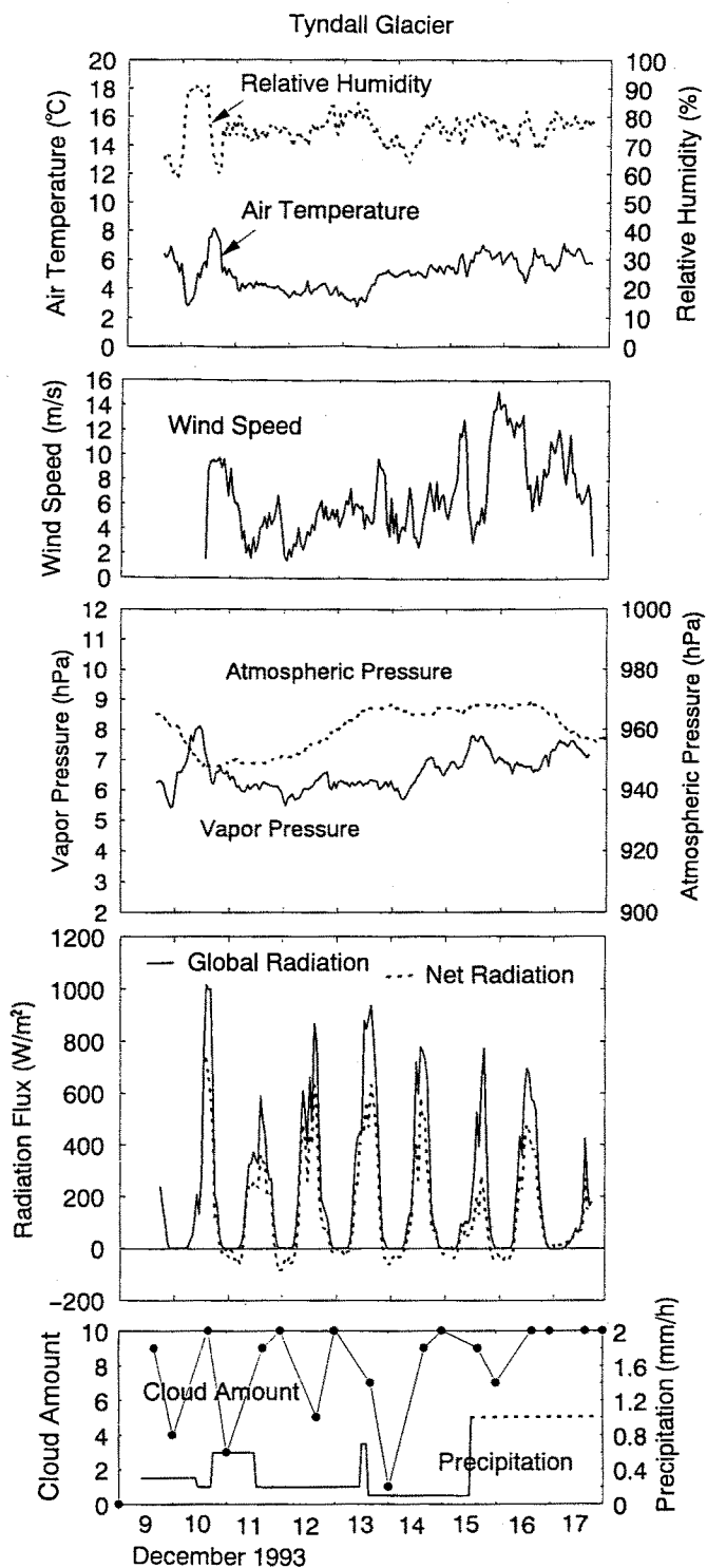
Fig. 2b. Variations in major meteorological elements at Tyndall Glacier during the observation period.
