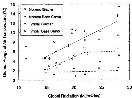
Fig. 7. Relationships between the daily global radiation and diurnal range of air temperature ( \Delta T ) on the glacier and at the Base Camp in Moreno and Tyndall glaciers. A dotted line is fitted to values at Moreno Glacier, a broken line is to Tyndall Glacier, and a solid line is to the base camps of the two glaciers.
