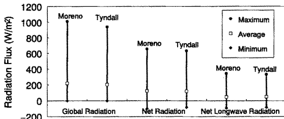
Fig. 4. The extremes and means of global radiation, net all wave radiation and net longwave radiation.
