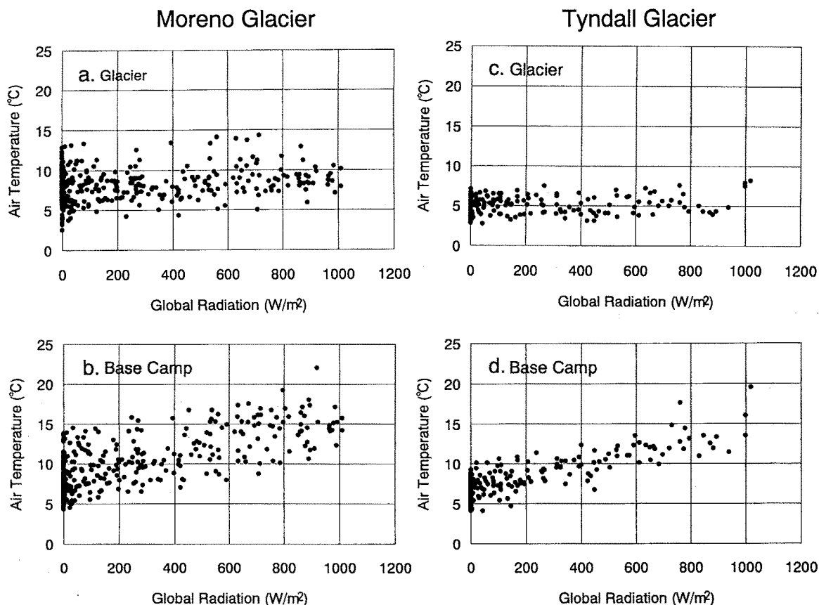
Fig. 8. Relationships between air temperature and global radiation on the glacier (a, c) and at the base camp (b, d) in Moreno and Tyndall glaciers.
