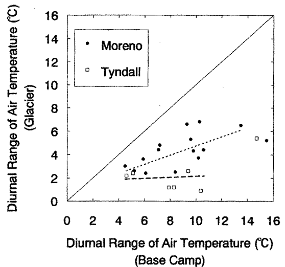
Fig. 6. Relationships between the diurnal range of air temperature ( \Delta T ) on the glacier and at the Base Camp in Moreno and Tyndall glaciers.
