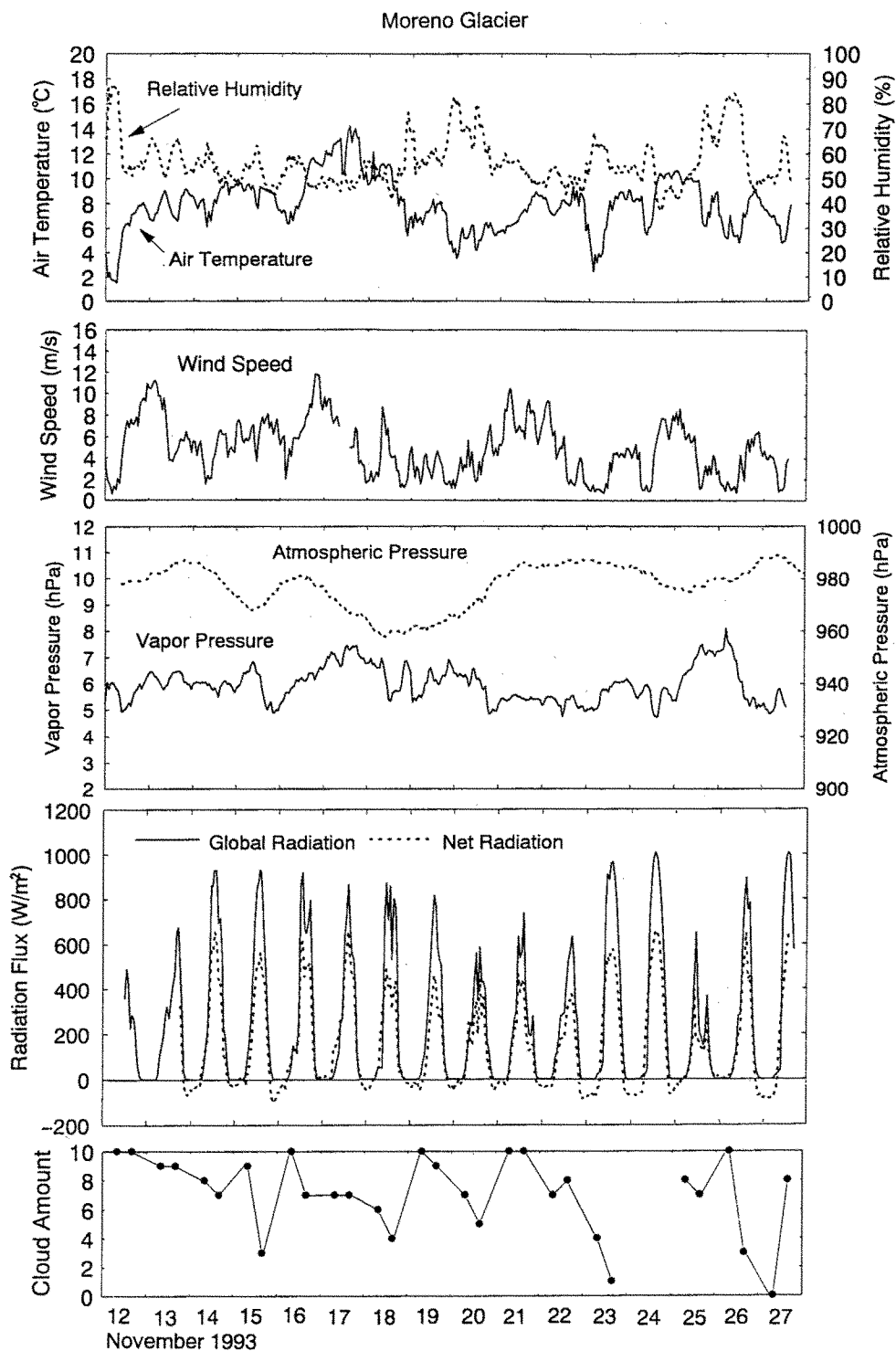
Fig. 2a. Variations in major meteorological elements at Moreno Glacier during the observation period.
