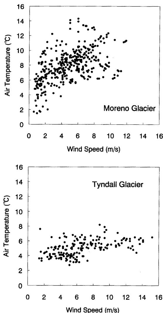
Fig. 9. Relationships between air temperature and wind speed on Moreno and Tyndall glaciers.
