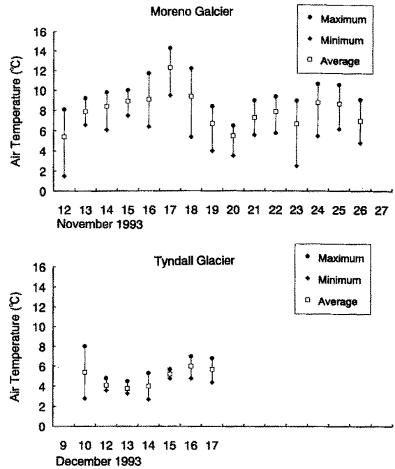
Fig. 5. The extremes and daily means of air temperatures.
