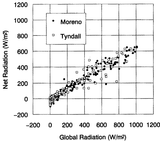
Fig. 3. Relationships between global radiation and net radiation on Moreno and Tyndall glaciers.
