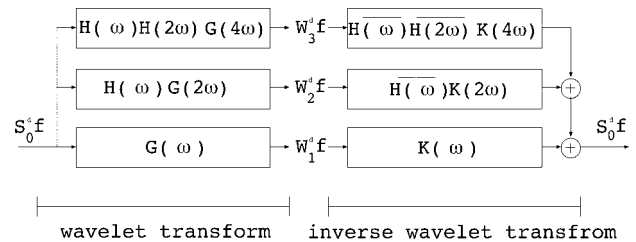
Fig.5 Parallel representation Frequency
