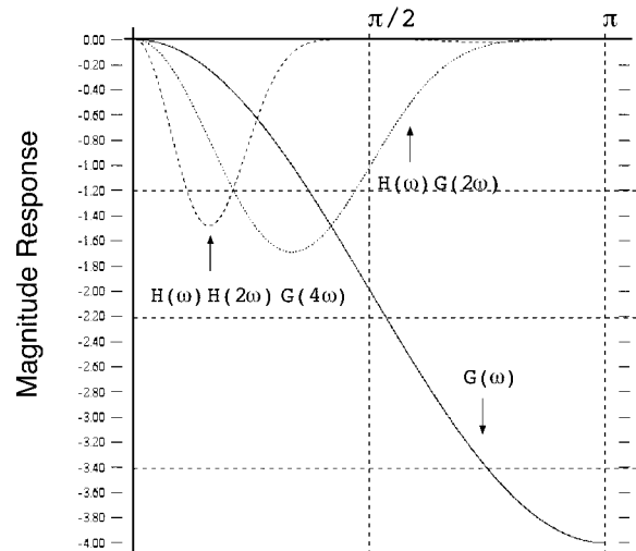
Fig.6 Frequency response of analysis filter
