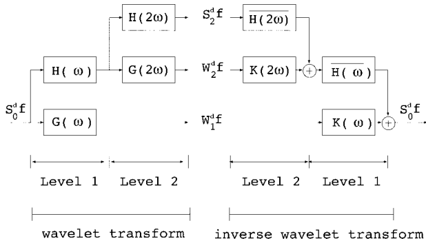
Fig.1 One-dimensional dyadic wavelet transform
