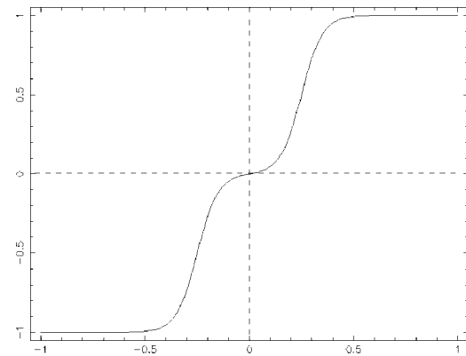
Fig.2 Non-linear filter ( b=0.25, c=20.0 )
