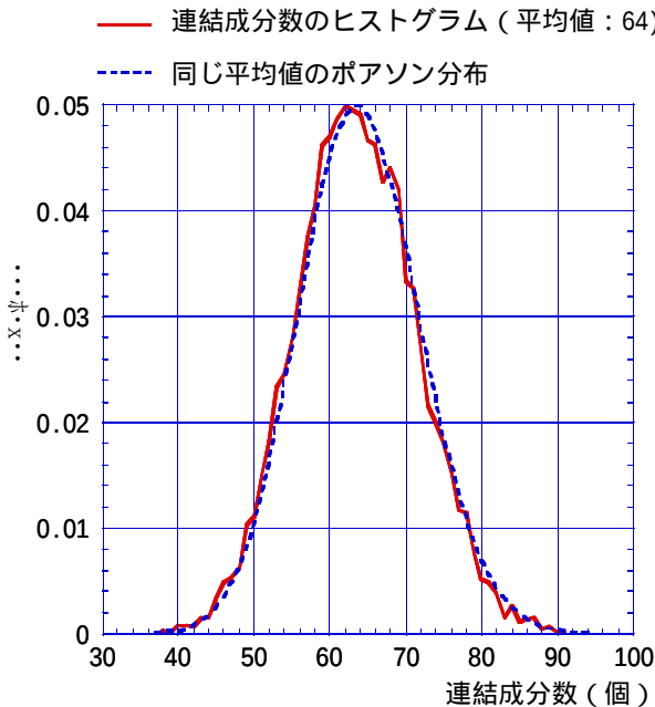
Fig.6 Distribution of number of connected components per an image.
