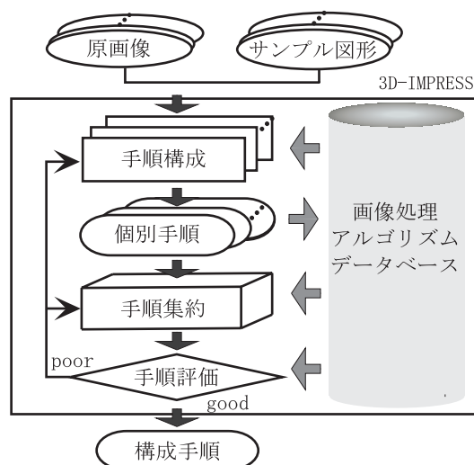
Fig.1 Outline of the 3D-IMPRESS.
