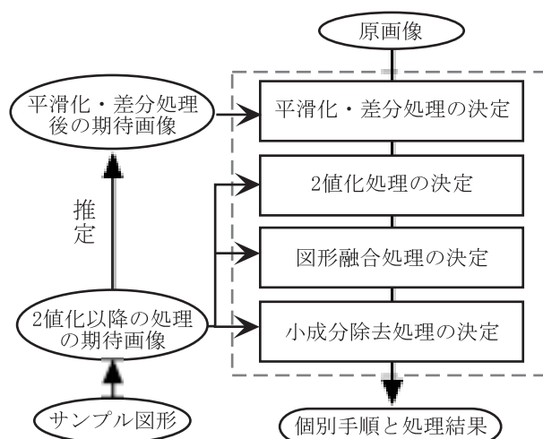
Fig.2 Flow of procedure construction for mass pattern extraction using a sample pair
