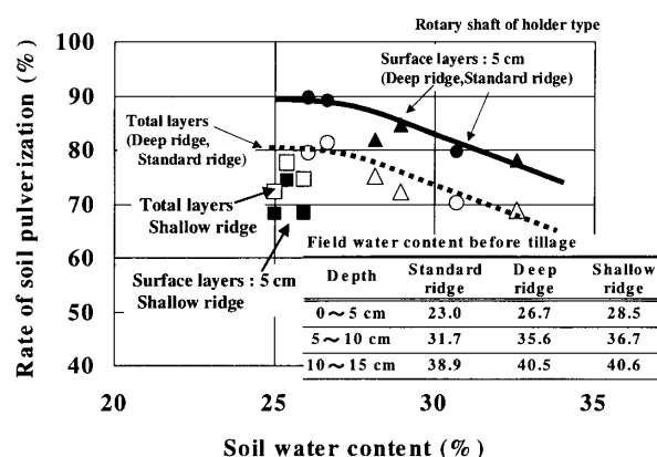
Fig. 9. Soil pulverization rate of ridges differing in tillage depth
