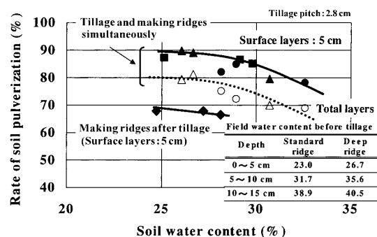
Fig. 8. Effect of simultaneous work on soil pulverization rate
