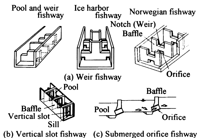
Fig. 1. Classification of artificial fishways (pool type)
