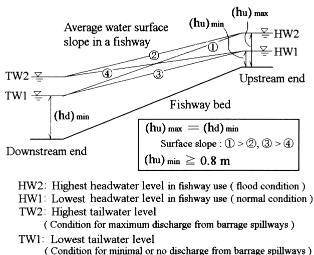
Fig. 11. Variation of average water surface slope in an orifice fishway (prototype size)
