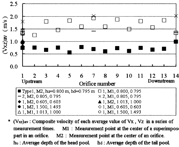
Fig. 6. Orifice velocity in the whole model (prototype size)
