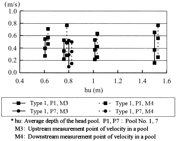
Fig. 8. (V_{xyz})_{max} , (V_{xyz})_{av} , (V_{xyz})_{min} in a pool of the whole model (Type 1, prototype size)
