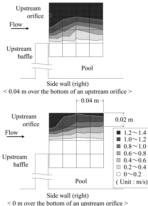
Fig. 5. (V_{xyz})_{av} contours downstream of the upstream orifice in the partial model (Prototype size, \Delta h = 0.094 m, h = 0.480 m, V_x = 1.21 m/s at the center of the orifice)
