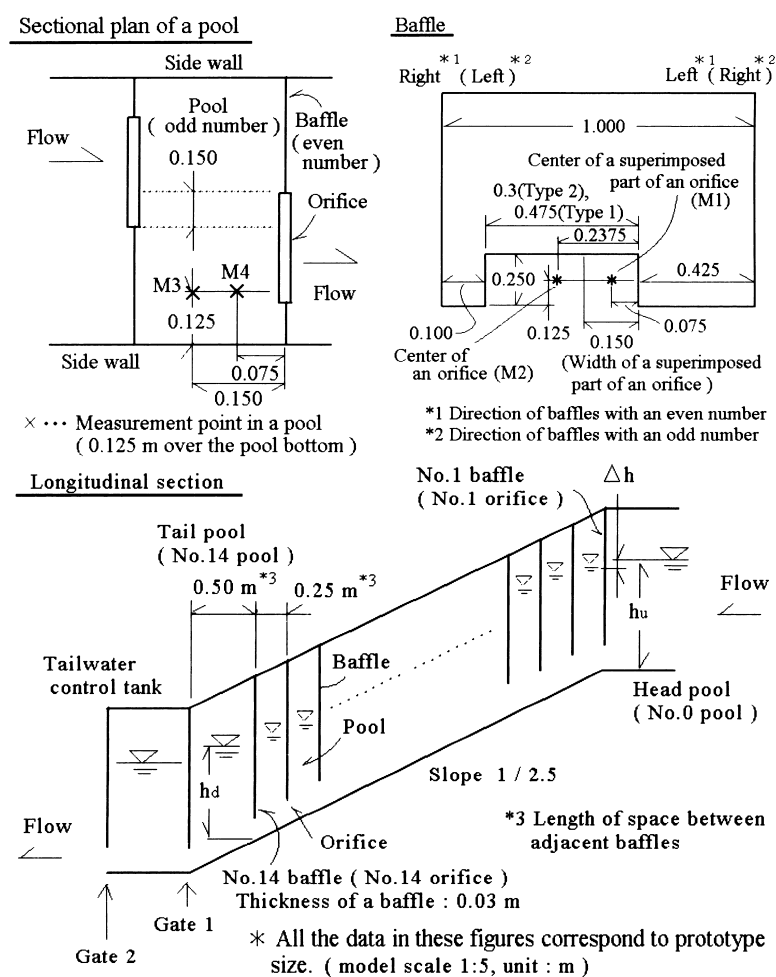
Fig. 4. Whole model of a submerged orifice fishway
