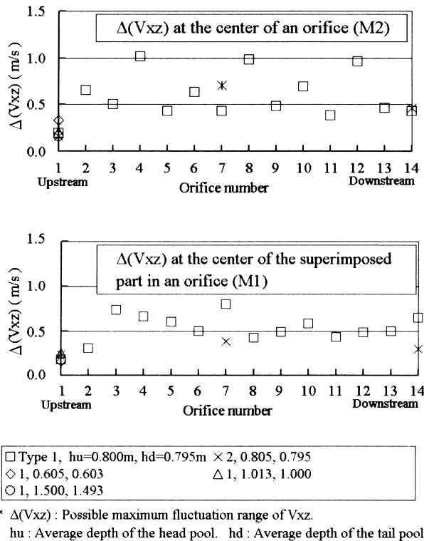
Fig. 7. Possible maximum fluctuation range of orifice velocity in the whole model (prototype size)
