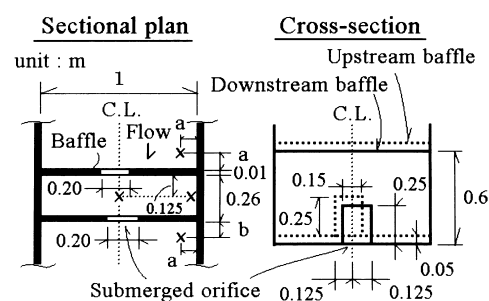
Fig. 2. Proposal for a fishway for various fish species and cost reduction
