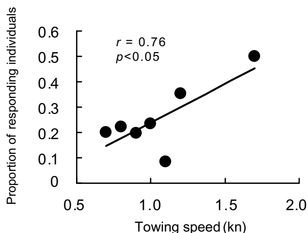
Fig. 4. Relationship between towing speed of the deep-sea video monitoring system on a towed sledge and proportion of responding individuals
