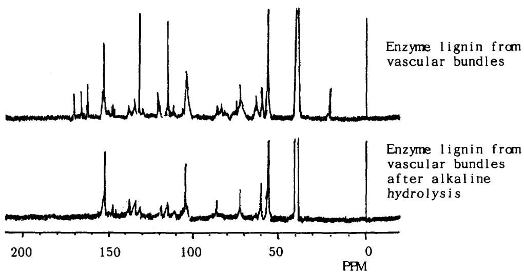
Fig. 5 ^{13}\text{C} -NMR spectra of enzyme lignin from matured trunk
