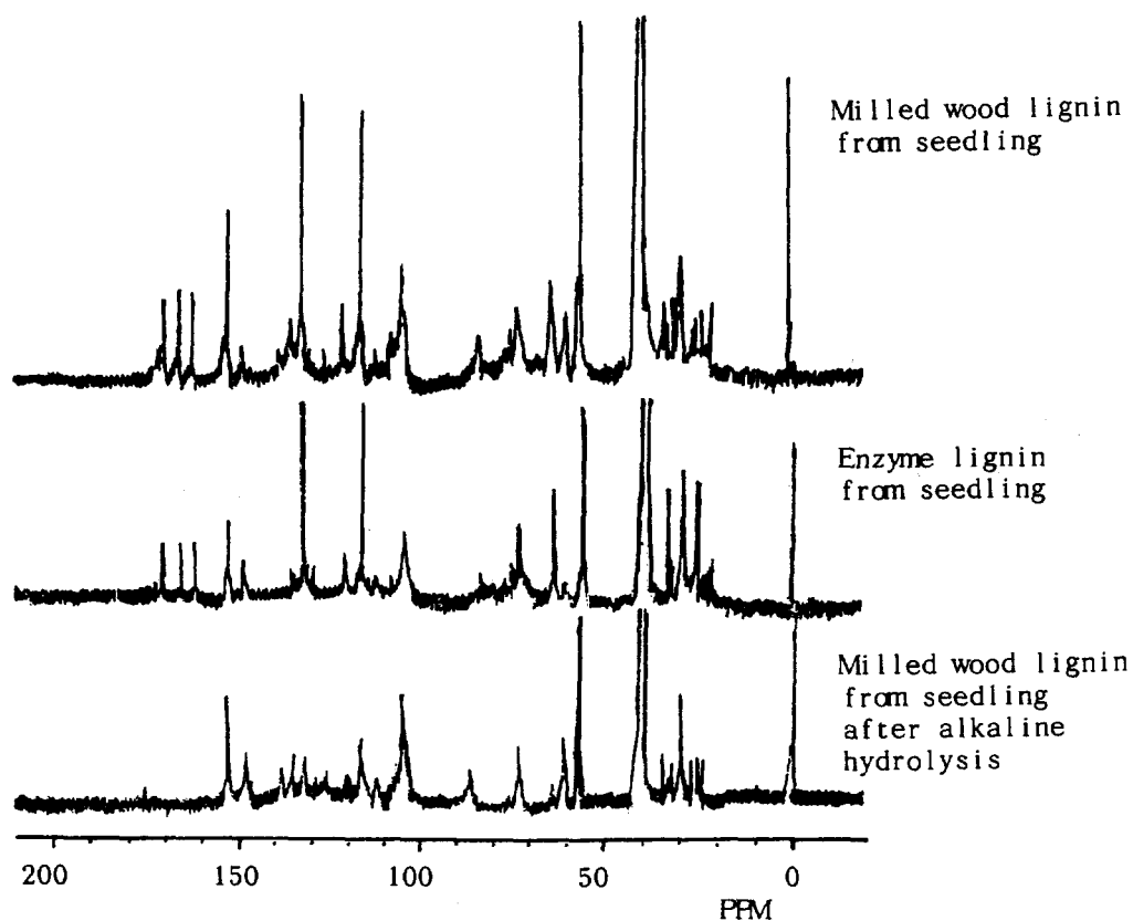
Fig. 4 ^{13}\text{C} -NMR spectra of seedling lignin
