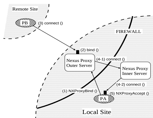
図 5 Nexus Proxy の通信メカニズム ( passive connection ) Fig. 5 Communication mechanism via the Nexus Proxy (passive connection).
