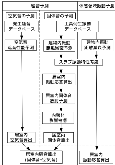
Fig. 8 騒音・振動予測フロー Flow of Noise and Vibration Simulation
