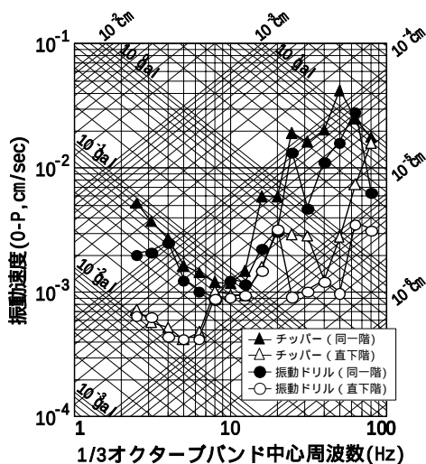
Fig. 6 発生振動周波数特性(事例1) Frequency Characteristics of Vibration
