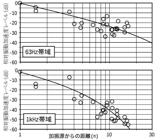
Fig. 4 振動の距離減衰実測結果と実験式推定値 Measured and Empirically Formulated Vibration Attenuation in Distance
