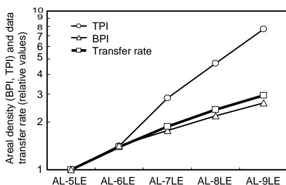
Figure 3 Areal density (BPI, TPI) and data transfer rate.
