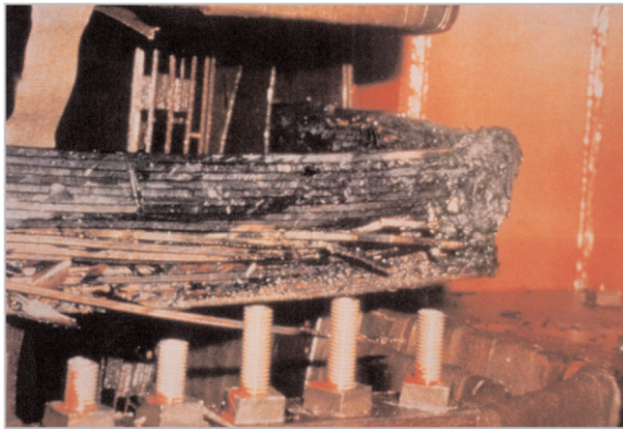
Fig.3 Coil inside an electric power transformer burnt out by space storm (Photograph courtesy of the United States Electric Power Research Institute)
