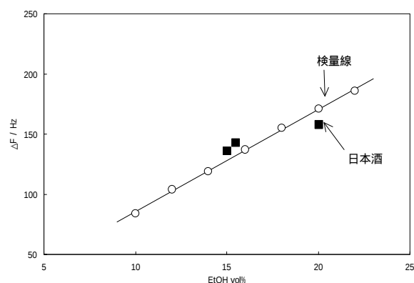
Figure 2. Sensor responses for aqueous ethanol solutions and sakes.
