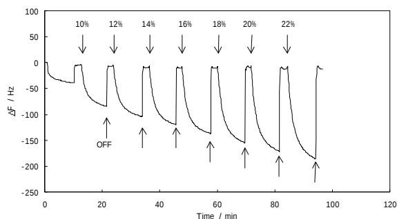
Figure 1. Frequency changes of a piezoelectric crystal coated with oleic acid ( \Delta F_M = 3.0 kHz) responding to aqueous ethanol solutions.
