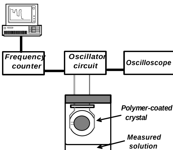
Scheme 1. Experimental setup for the piezoelectric sensor system.
