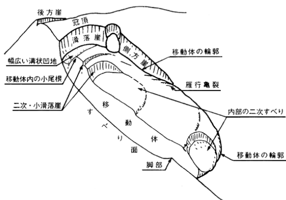
図1 地すべり地形の模型図 Fig. 1 Schematic figure of landslide landform.
