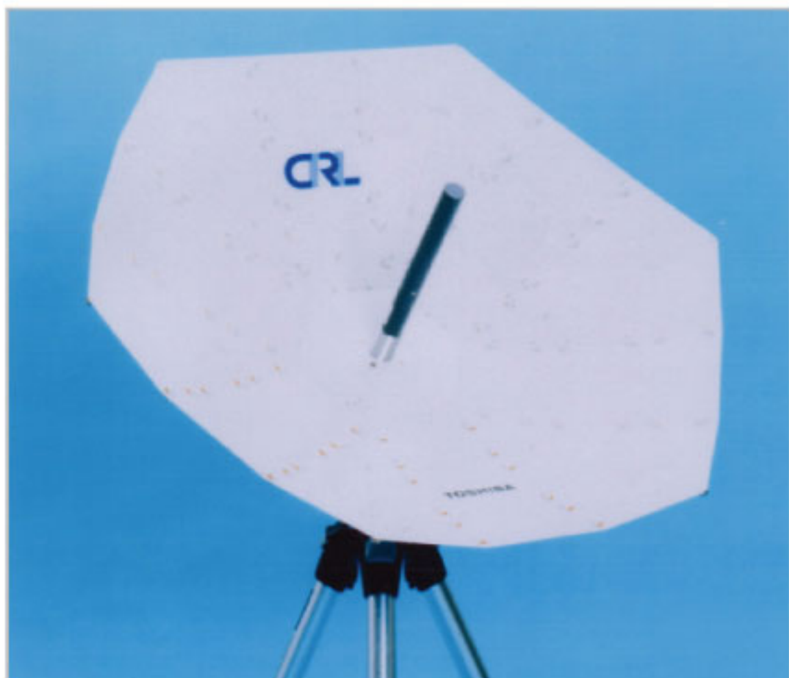
Fig.5 Deployed prototype
