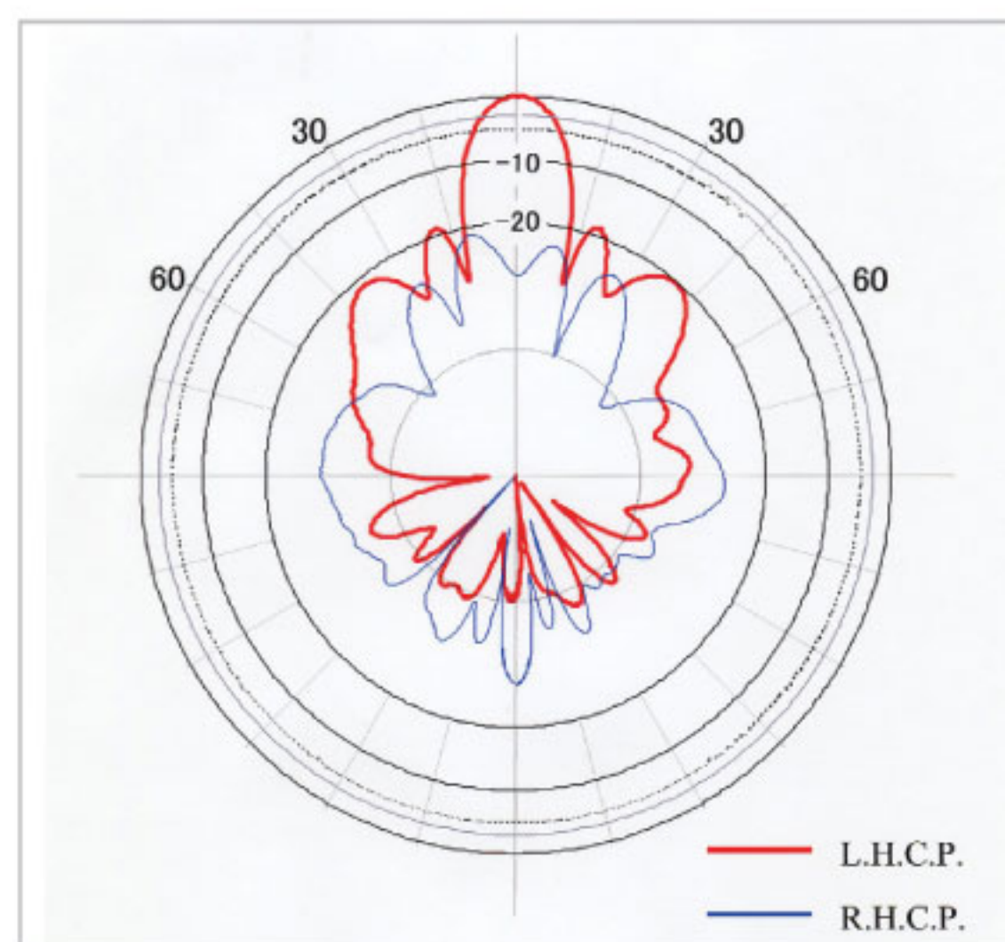
Fig.8 Prototype radiation pattern
