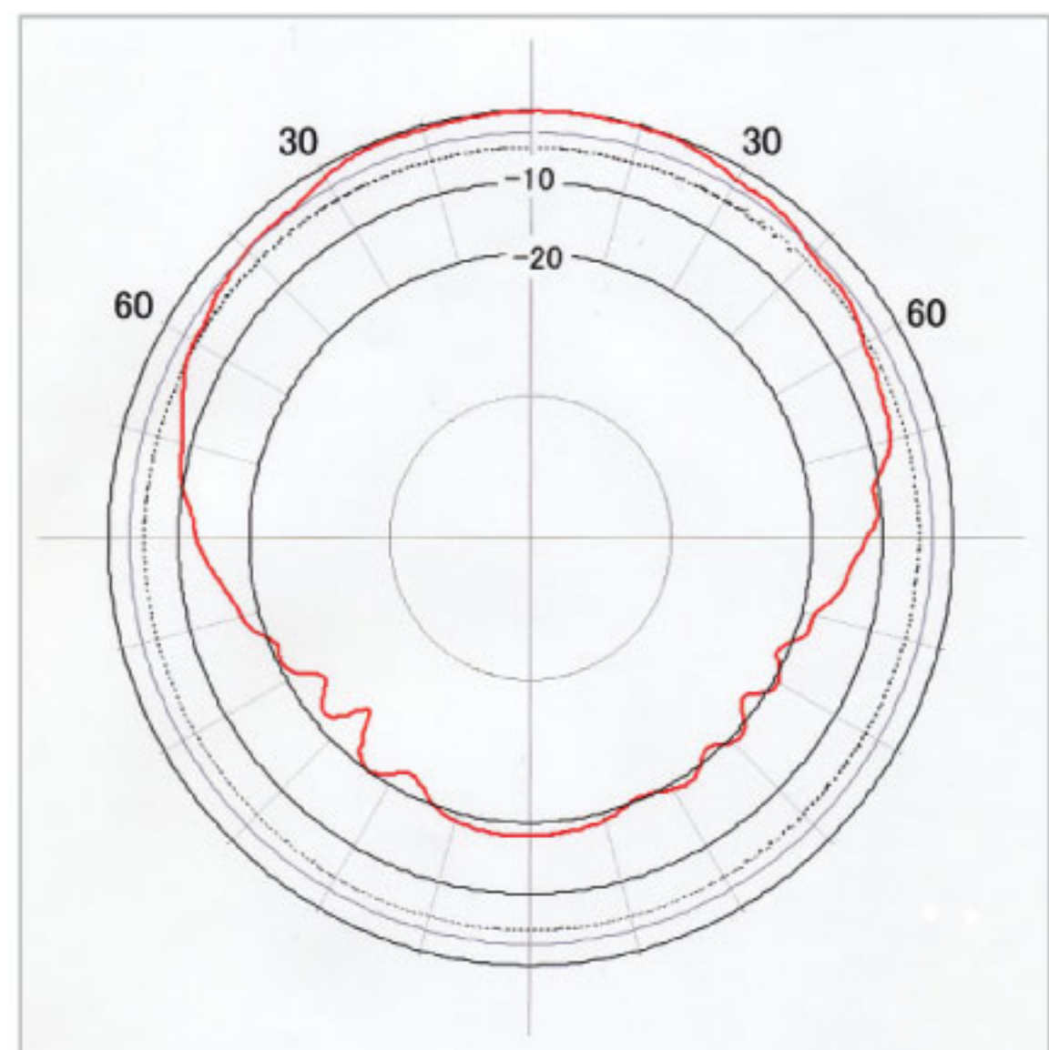
Fig.4 Radiation pattern of the quadrifilar helix antenna
