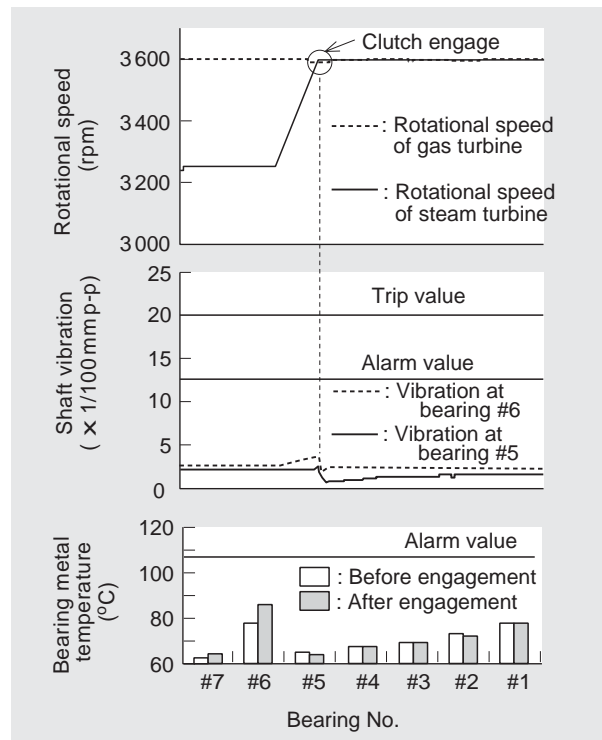
Fig. 9 Operation of turbine using SSS clutch Indicates changes in shaft vibration and bearing metal temperature before and after clutch engagement.
