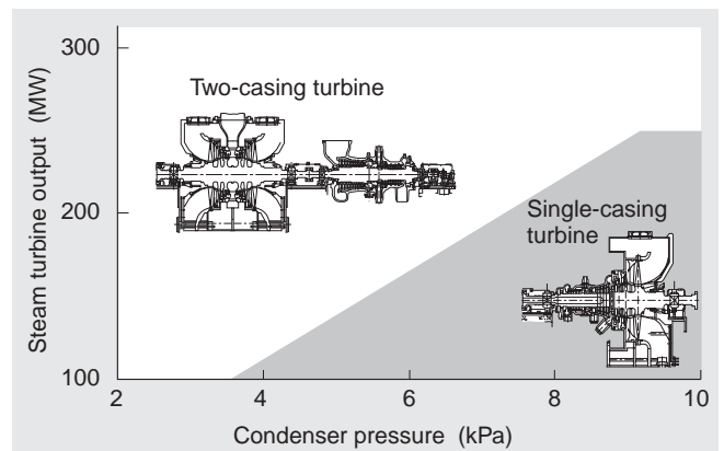
Fig. 1 Steam turbine capacity and casing arrangement Indicates the applicable range of output and condenser pressure for single-casing turbines.
