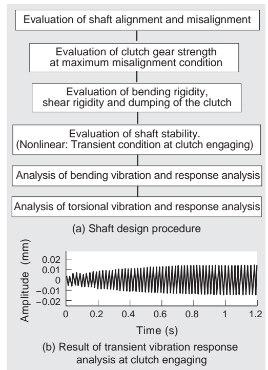
Fig. 8 Design of shaft system including SSS clutch
