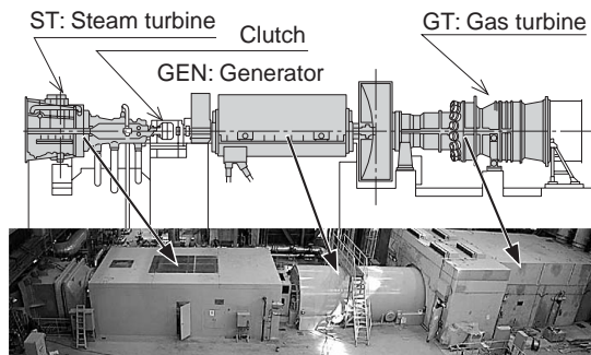
Fig. 7 Turbine shaft arrangement applying SSS clutch Clutch is installed between steam turbine and generator.
