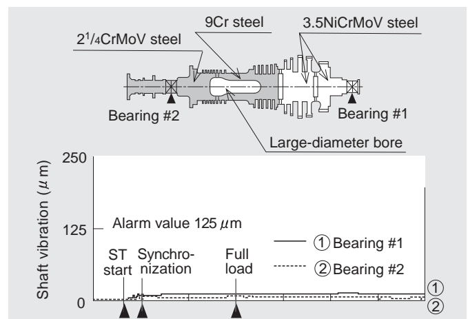
Fig. 4 Operations of large-bore hetero-material welded rotor at T-point Indicates small shaft vibration even at quick start.
