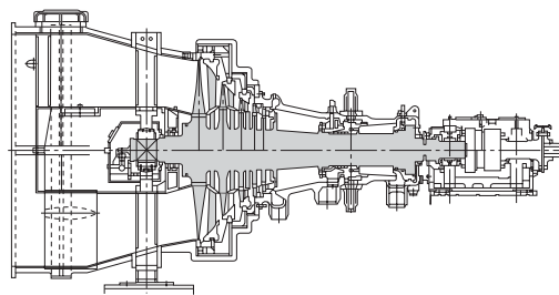
Fig. 6 Large-capacity axial-exhaust single-casing reheat turbine 3000 rpm, 48-inch steel blade used for last-stage blade.
