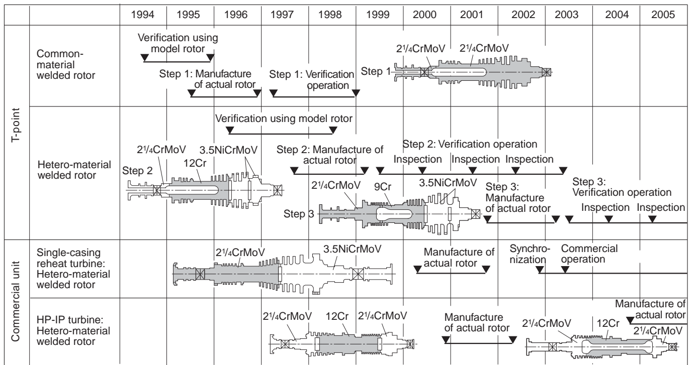
Fig. 3 Application of welded rotor to actual turbine
