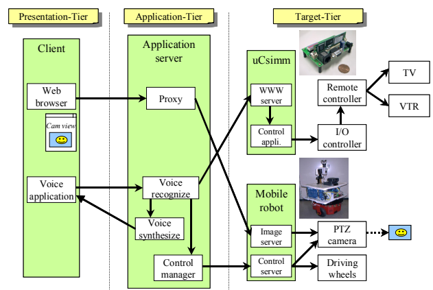
Fig.10 System configuration
