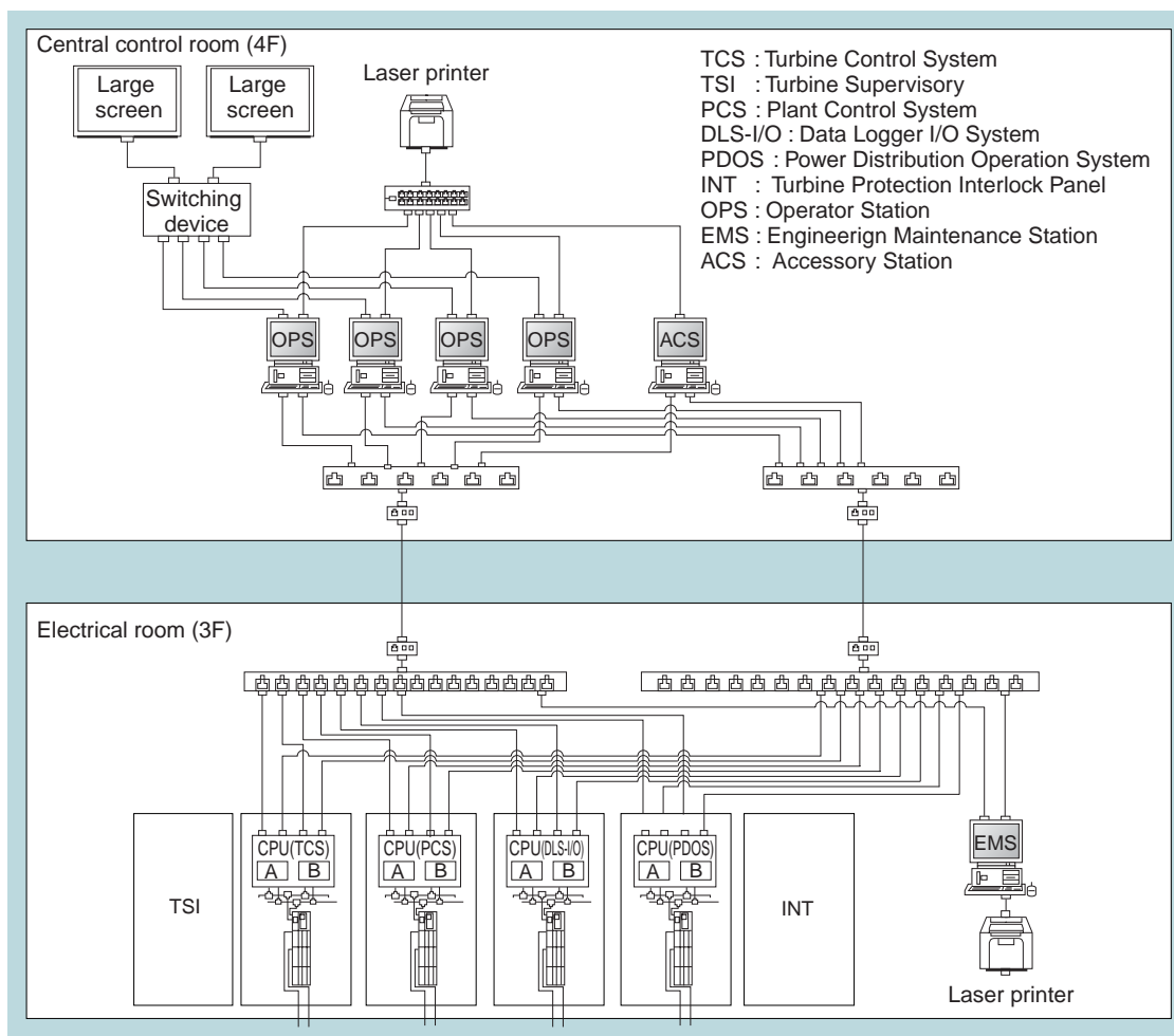
Fig. 6 Control system configuration
