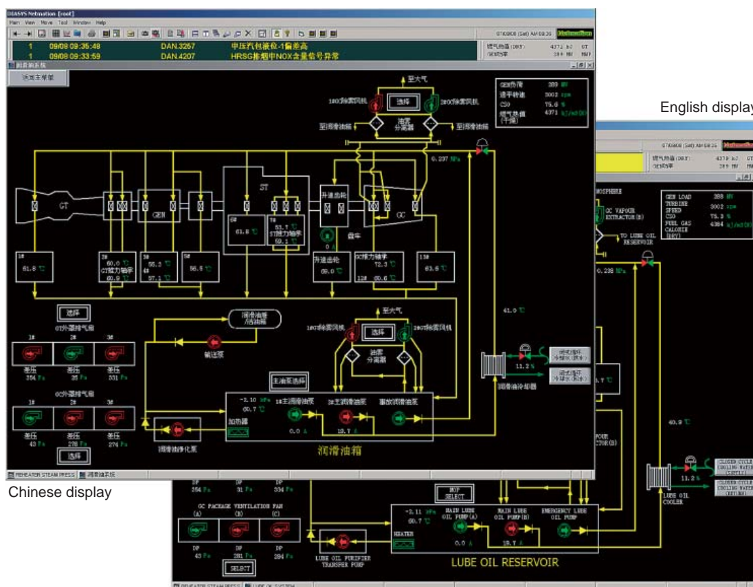
Fig. 8 Sample system schematic screens in both Chinese and English
