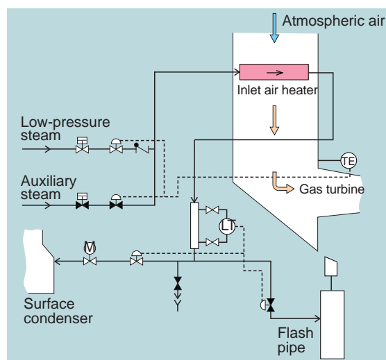
Fig. 5 Outline schematic of inlet air heating system
