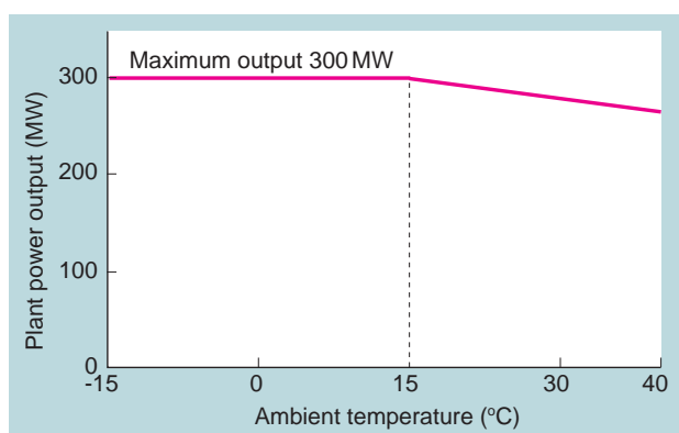
Fig. 4 Plant output characteristics
