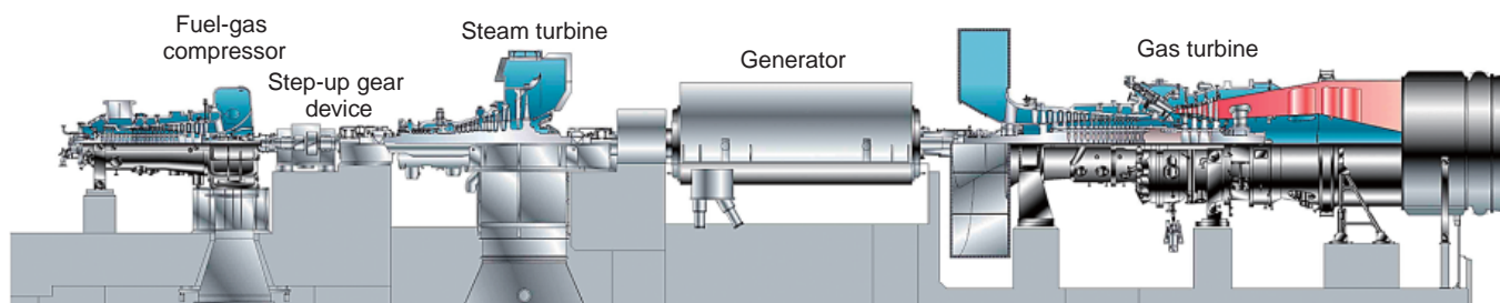
Fig. 3 Longitudinal sectional drawing of complete assembly
