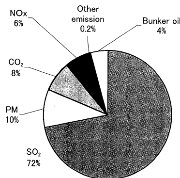
Fig.15 Effect of the fuel and emissions caused by cargo unloading at port on the environmental impacts
