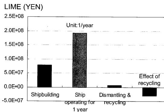
Fig.20 LIME's integrated single index for environmental impact of ship's life cycle
