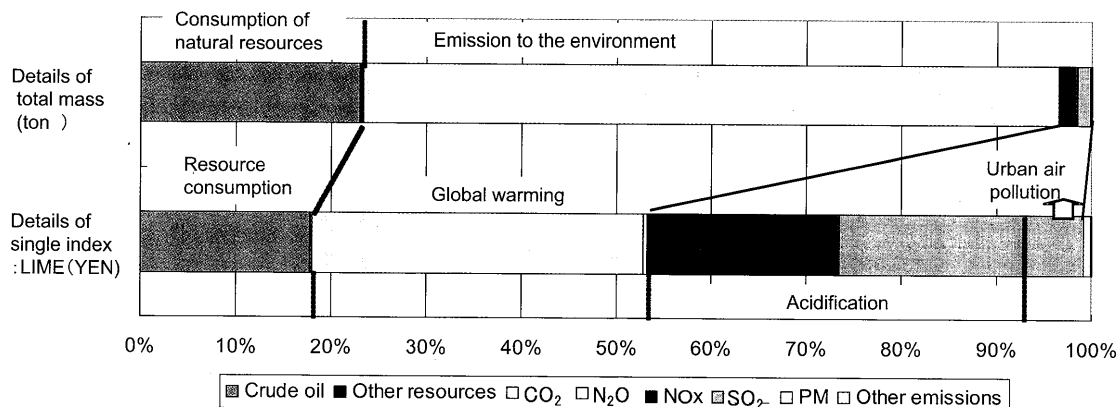
Fig.13 Effect of load items caused by ship operating. Upper horizontal bar: share of total mass including consumption or emissions of load items Lower horizontal bar: share of environmental impacts based on LIME
