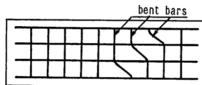
Fig. 2 Arrangement of reinforcement of slab No.4
