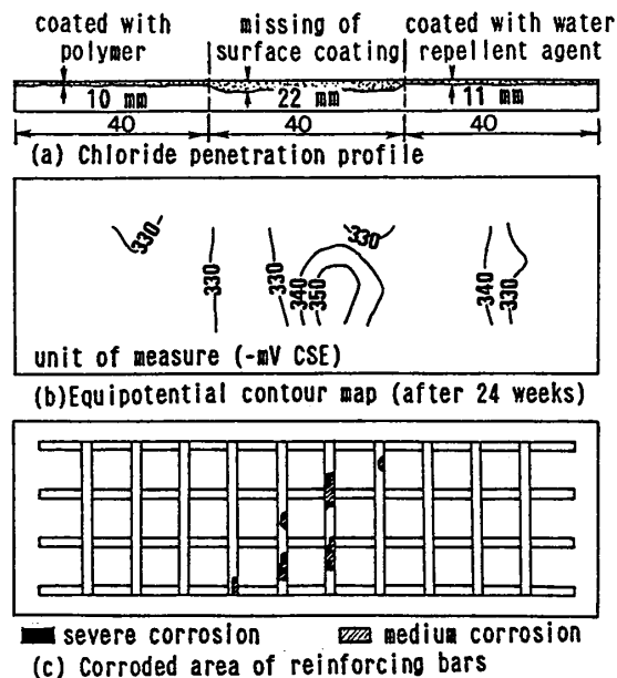
Fig. 13 Influence of surface coating on chloride penetration, equipotential contour map, and corroded area of reinforcing bars
