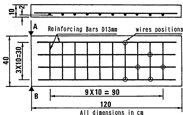
Fig. 1 Details of test specimen
