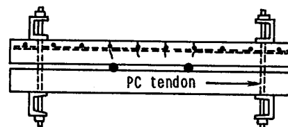
Fig. 2 Arrangement of reinforcement of slab No.4
