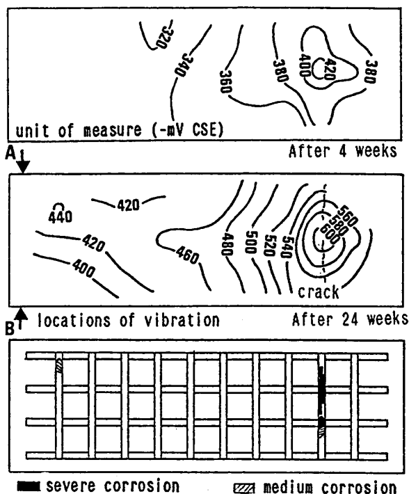
Fig. 7 Equipotential contour map and corroded areas of reinforcing bars in slab No.2
