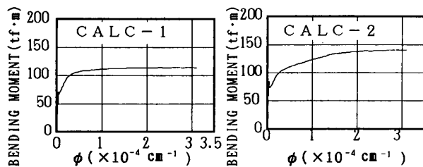
図-14 M-φ (CALC-1、CALC-2)
