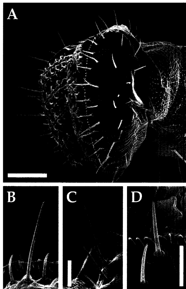
Fig. 1. Morphology of the labellar chemosensilla in Drosophila . Three types of sensillum, L-, I- and S-type, are visible on the labellum (Shanbhag et al. , 2001). (A) Lateral view of the left lobe of a labellum. Anterior is top and dorsal to the right. Chemosensilla are arranged in four rows oriented in the anterior-posterior axis (Falk et al. , 1976; Ray et al. , 1993). The S-type sensilla are in the most ventral area and the I-type sensilla are located in the most dorsal area. Enlarged images of L-type (B), I-type (C) and S-type sensilla (D). B–C are shown in the same scale. Scale bars represent 40 µm (A) and 10 µm (C and D).
