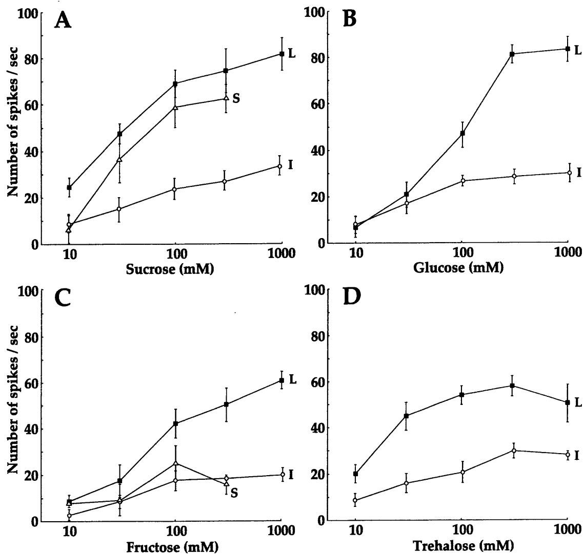
Fig. 6. Dose-response curves of the L-, S- and I-type sensilla to sucrose (A), glucose (B), fructose (C) and trehalose (D). Vertical bars represent standard errors. Responses of the L-, I- and S-type sensilla are shown as closed squares, open circles and open triangles, respectively. Each point was calculated from 40-52 recordings from L-type sensilla, 35-45 recordings from I-type sensilla and 10-21 recordings from S-type sensilla using 44 flies.
