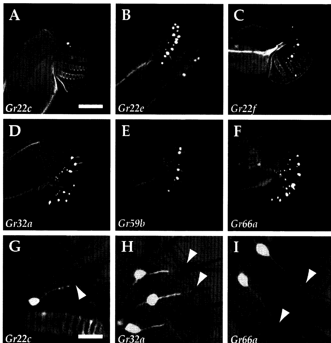
Fig. 3. Expression of Gr genes monitored by Gr promoter-Gal4/UAS-GFP. Images captured at 2 \mu m intervals for a 30–40 \mu m-thick section of a labellum were overlaid. (A–F) Each Gr promoter-Gal4 line shows a different expression pattern. In all lines, two levels of GFP expression were observed. A–F and G–I are each shown in the same scale. (G–I) Overlaid images of fluorescent and Nomarski images. Arrowheads show the identified sensilla. Scale bar in A is 40 \mu m and in G is 10 \mu m.
