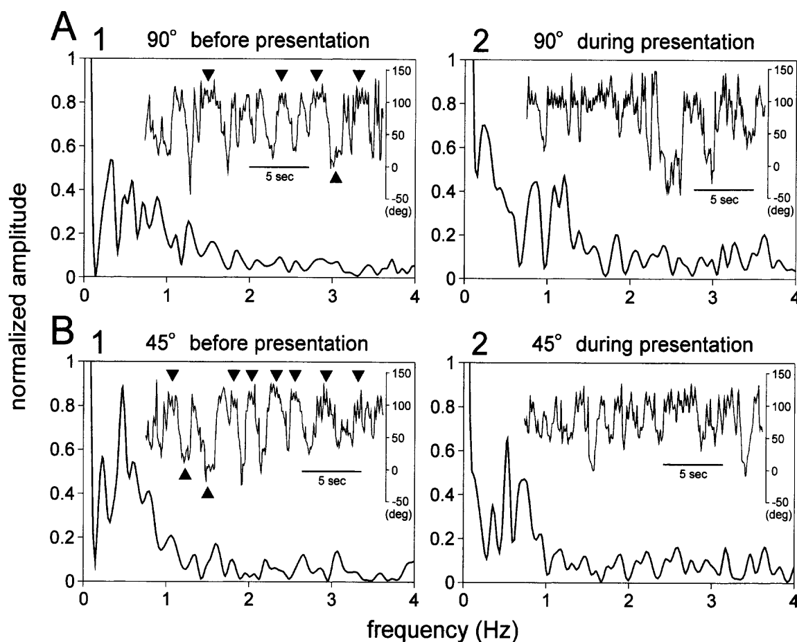
Fig. 3. Amplitude-frequency relationships of horizontal antennal movements after the S-HP ablation. FFT spectra before (1) and during (2) object presentations at 90^\circ (A) and 45^\circ (B). The original data were derived from those shown in the Fig. 1. The “over-swing” movements of treated antenna are represented clearly by increases in low frequency (<1 Hz) components in all four spectrograms (compare with the spectra in Fig. 2). Arrowheads in insets show small tremble-like cycles around the extreme positions.
