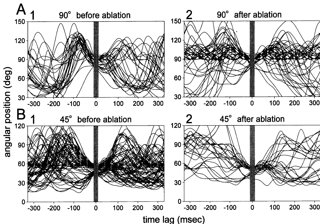
Fig. 4. Trajectories of horizontal antennal movements before and after contacts with test objects. Time zero means the instant of antennal contact. A. Superimposed trajectories before (1) and after (2) the S-HP ablation in the object presentations at 90^\circ for 20 sec. After the ablation, the I-P pattern almost disappeared. Number of contacts: 31 before the ablation, 47 after the ablation. B. Superimposed trajectories in the object presentations at 45^\circ for 20 sec. Though the number of contacts decreased from 77 (before ablation) to 26 (after ablation), the contact patterns themselves did not basically change. Data points for the trajectories were connected with spline curvature methods.
