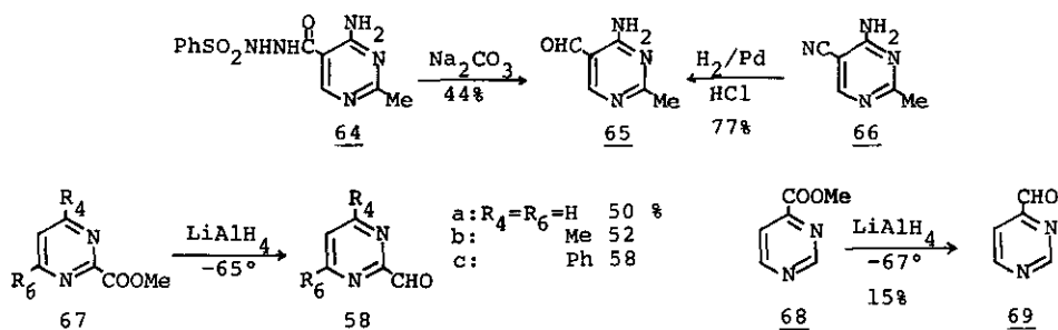
Scheme 13
